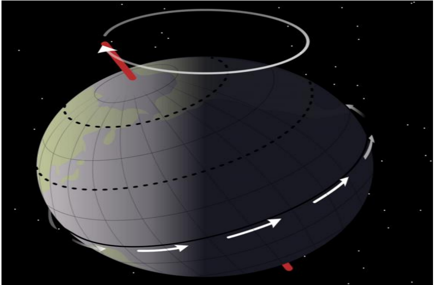
Earth Is Tilted: 23.44 degrees
